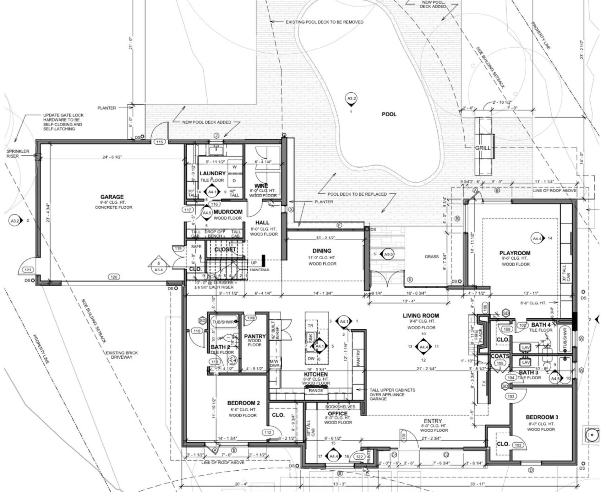
1 ENTRY LEVEL PLAN 3/16" = 1'-0"
